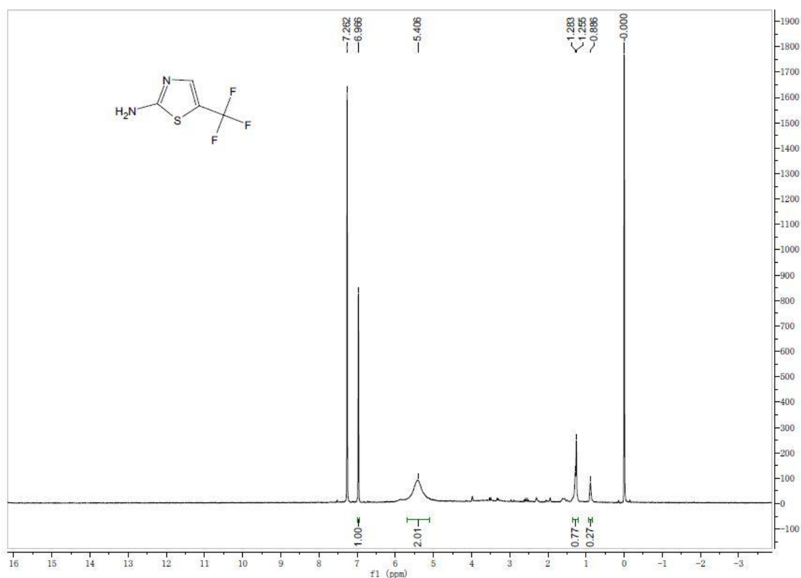
Figure S1. 1 H NMR spectrum (400 MHz, CDCl 3 ) of 5-(trifluoromethyl)-2-thiazolamine.
