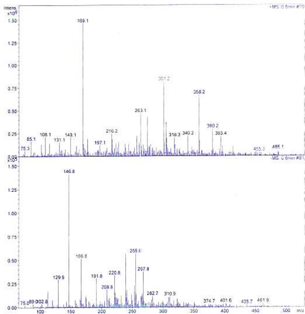
Figure S2. Mass spectrum of compound 5-(trifluoromethyl)-2-thiazolamine.
