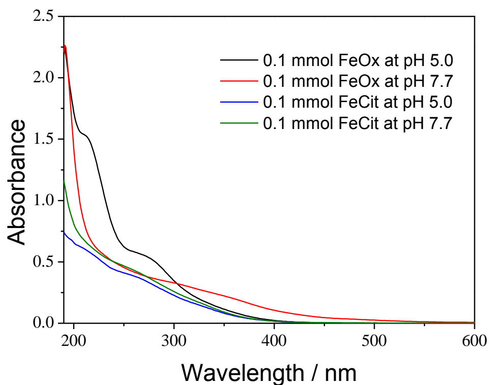
Figure S1. Absorption spectrum of aqueous solutions iron citrate (FeCit) and iron oxalate (FeOx) at pH 5.0 and 7.7.
