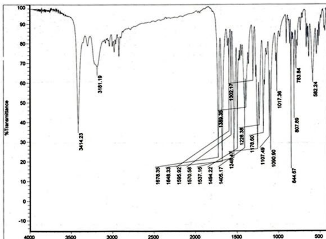
Figure S9. IR spectrum (KBr) of 2-[2'-(2-(1,3-diphenyl-1 H -pyrazol-4-yl)thiazolidine-5-one)acetyl-aminomercapto] benzimidazole ( 8a ).
