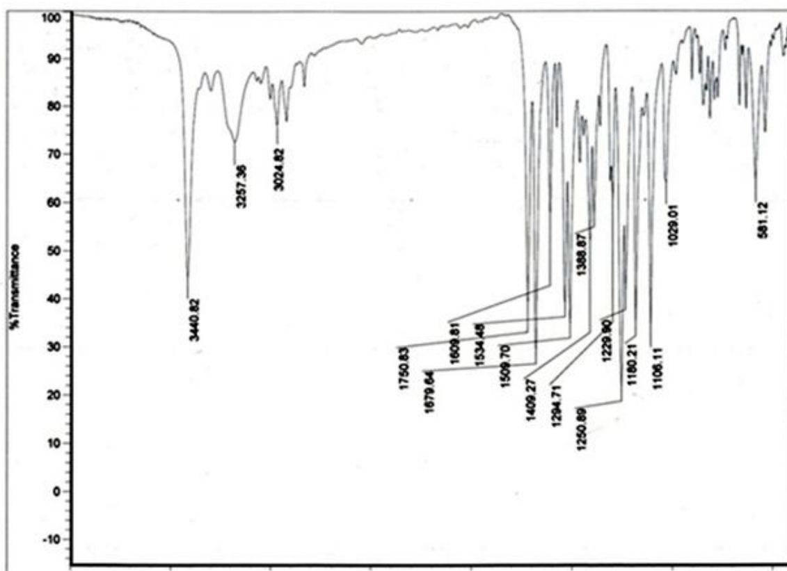
Figure S5. IR spectrum (KBr) of 2-[4'-(1,3-diphenyl-1 H -pyrazol-4-yl)-3'-chloro-2'-oxoazetidine]hydrazinobenzimidazole ( 5a ).
