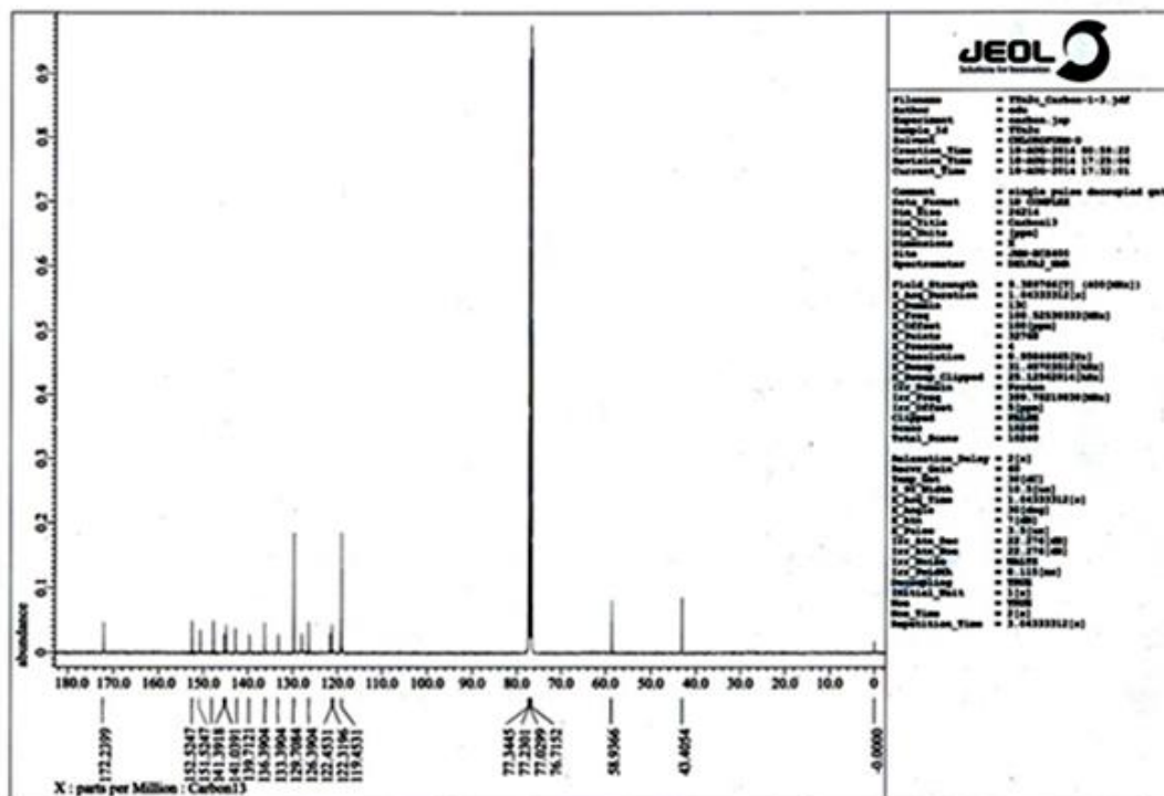
Figure S7. ^{13}\text{C} NMR spectrum (100 MHz, \text{CDCl}_3 ) of 2-[4'-(1,3-diphenyl-1 H -pyrazol-4-yl)-3'-chloro-2'-oxoazetidine]hydrazinobenzimidazole ( 5a ).
