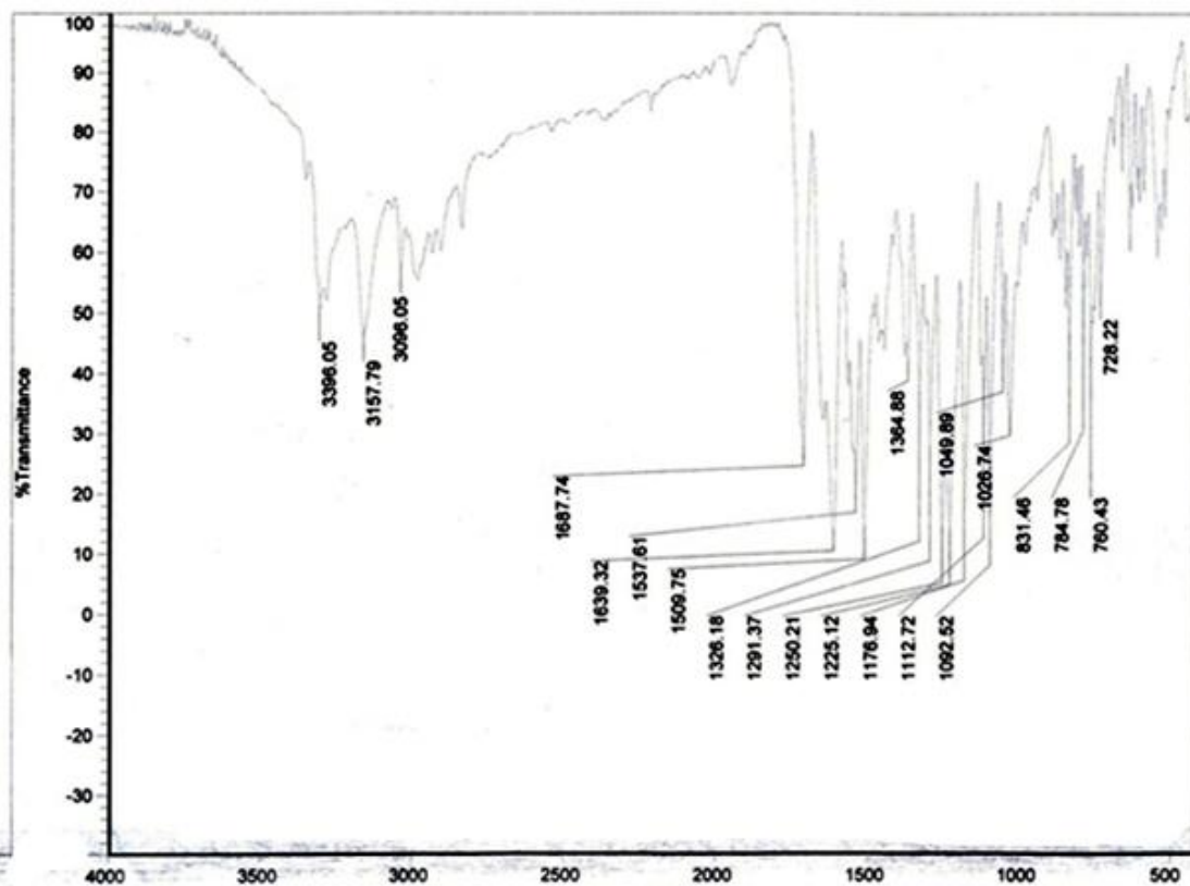
Figure S13. IR spectrum (KBr) of (benzimidazol-2-ylsulfanyl)acetic acid ((1,3-diphenyl-1' H -pyrazol-4-yl)methylidene) hydrazide ( 11a ).
