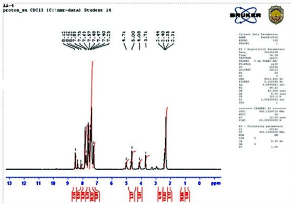
Figure S10. ^1\text{H} NMR spectrum (400 MHz, \text{CDCl}_3 ) of 2-[2'-(2-(1,3-diphenyl-1 H -pyrazol-4-yl)-thiazolidine-5-one)acetylaminomercapto] benzimida-zole ( 8a ).
