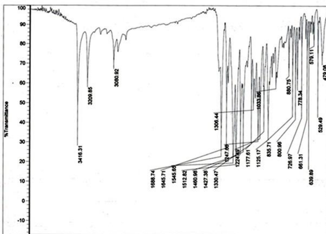
Figure S11. IR spectrum (KBr) of 2-[2'-(4-(1,3-diphenyl-1 H -pyrazol-4-yl)-3-chloro-2-oxo-azetidine)acetylaminomercapto]benzimidazole ( 9a ).
