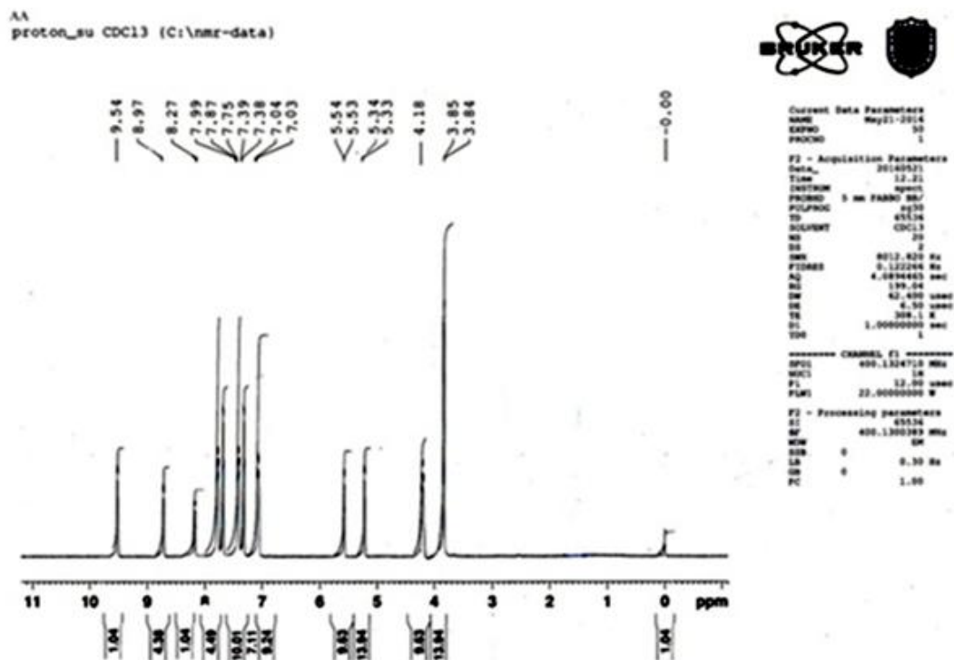
Figure S12. ^1\text{H} NMR spectrum (400 MHz, \text{CDCl}_3 ) of 2-[2'-(4-(1,3-diphenyl-1 H -pyrazol-4-yl)-3-chloro-2-oxoazetidine)acetylaminomercapto]benzimidazole ( 9a ).
