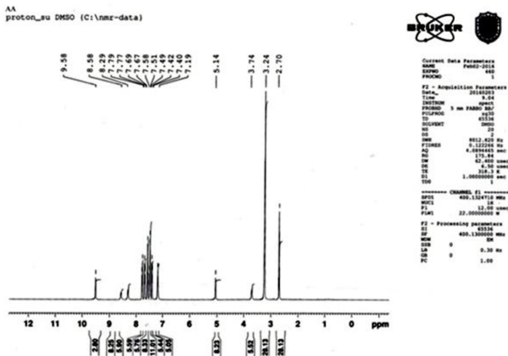
Figure S4. ^1\text{H} NMR spectrum (400 MHz, \text{DMSO-}d_6 ) of 2-[2'-(1,3-diphenyl-1 H -pyrazol-4-yl)thiazolidine-5'-one]hydrazinobenzimidazole ( 4a ).
