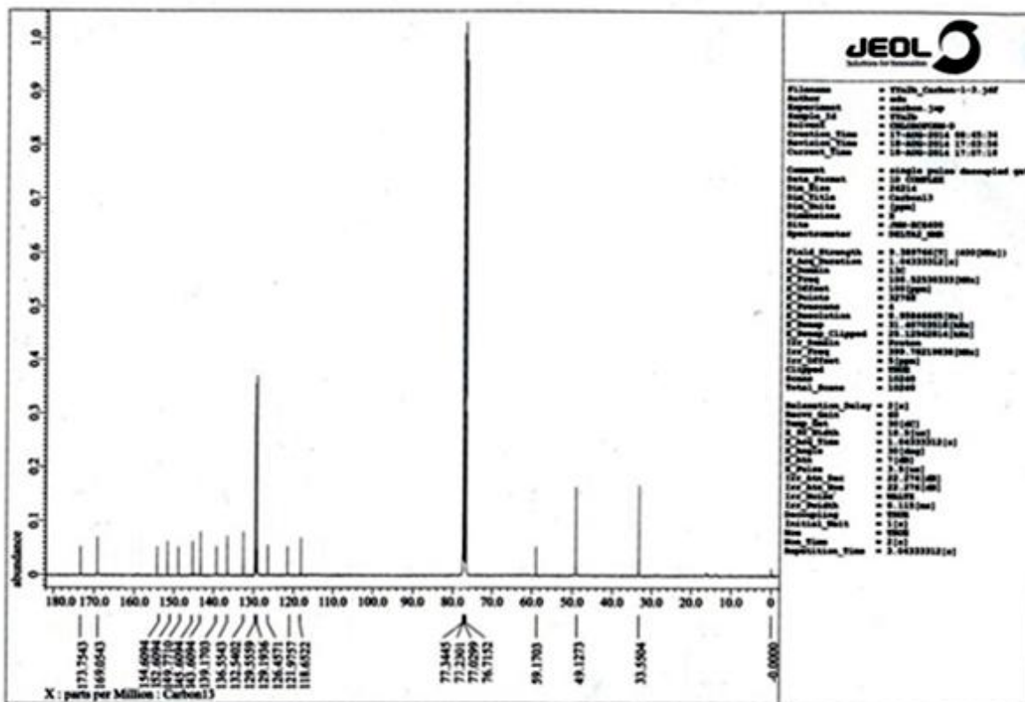
Figure S16. ^{13}\text{C} NMR spectrum (100 MHz, \text{CDCl}_3 ) of 1-[(benzimidazol-2''-yl)thioacetamidyl]-3-chloro-4-(1',3'-diphenyl-1' H -pyrazol-4'-yl)azetidin-2-one ( 13a ).
