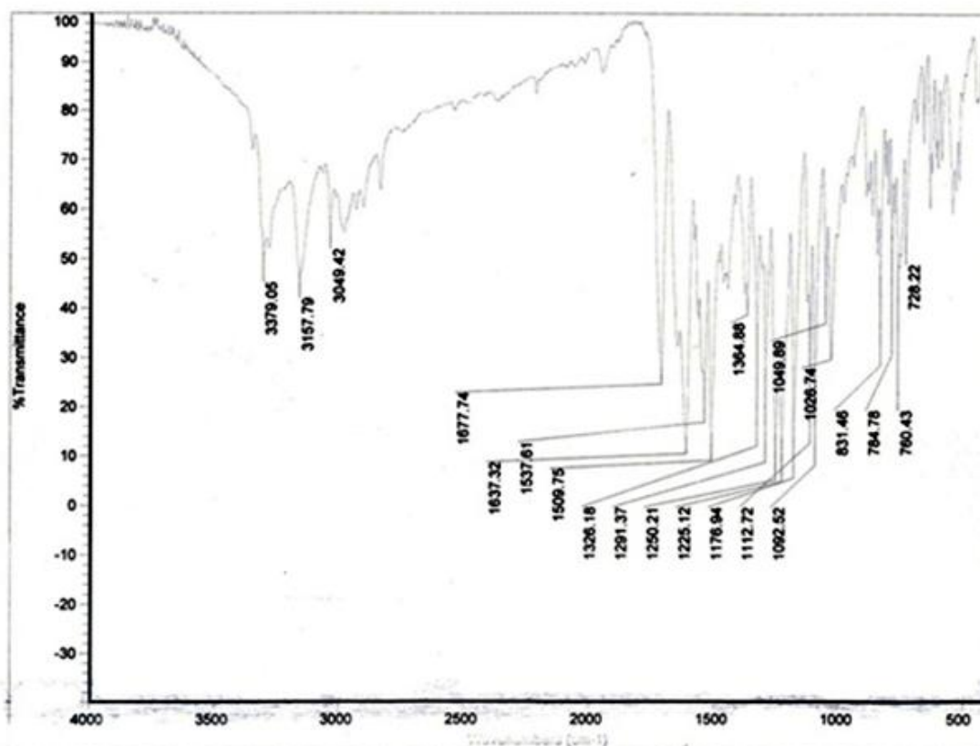
Figure S8. IR spectrum (KBr) of benzoimidazol-2-yl 2-(2-((1,3-diphenyl-1 H -pyrazol-4-yl)methylene)hydrazinyl)ethanethioate ( 7a ).
