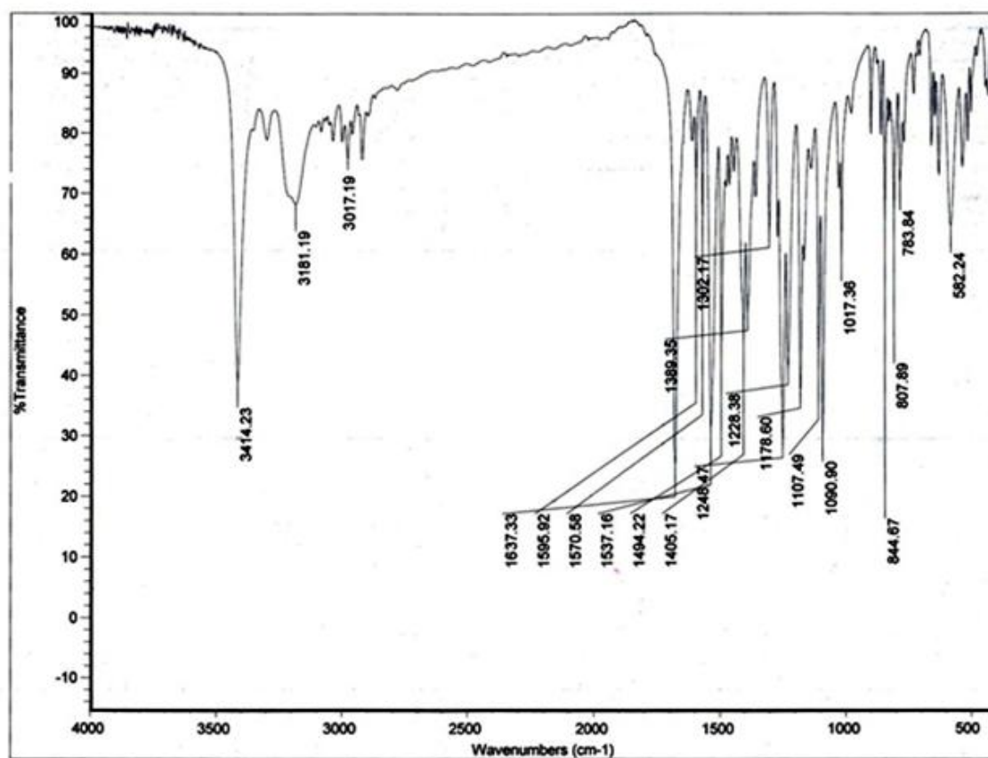
Figure S1. IR spectrum (KBr) of 2-((1,3-diphenyl-1H-pyrazol-4-yl)methylene)hydrazinyl)-1H-benzimidazole (3a).
