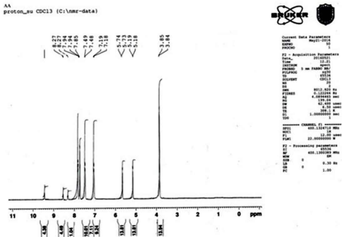
Figure S6. ^1\text{H} NMR spectrum (400 MHz, \text{CDCl}_3 ) of 2-[4'-(1,3-diphenyl-1 H -pyrazol-4-yl)-3'-chloro-2'-oxoazetidine]hydrazinobenzimidazole ( 5a ).
