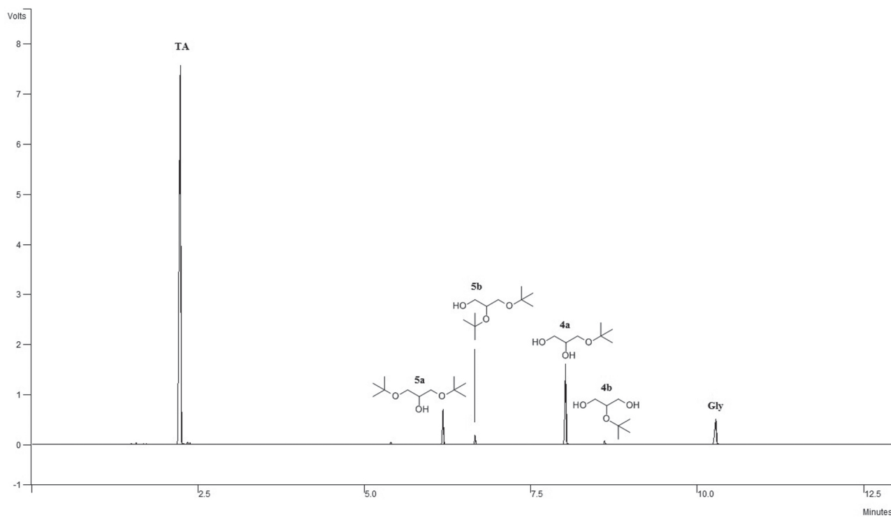
Figure 5. Chromatogram profile of the reaction medium of the etherification of glycerol with t -butanol. Peak identification: t -butanol (TA); 1,3-di- tert -butoxy-propan-2-ol ( 5a ); 2,3-di- tert -butoxy-propan-1-ol ( 5b ); 3- tert -butoxy-propane-1,2-diol ( 4a ); 2- tert -butoxy-propane-1,3-diol ( 4b ); glycerol (Gly).
