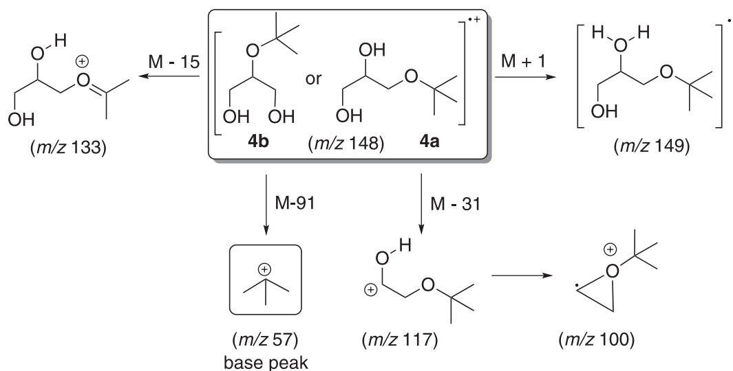
Figure 6. Proposed fragmentation pathway for monosubstituted ethers 4a and 4b .
