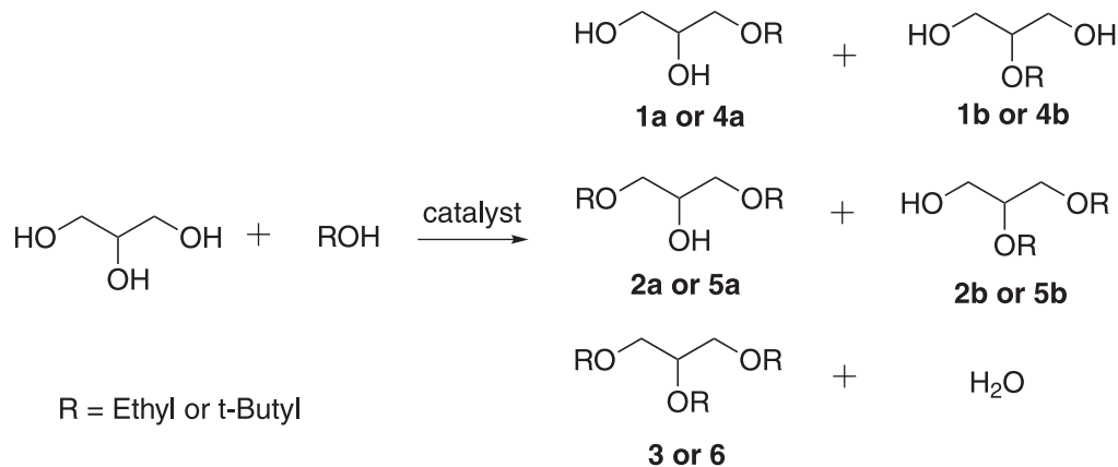
Figure 1. Products of the glycerol and ethanol or t -butanol etherification reaction in the presence of acid catalyst. 1a : 3-ethoxy-propane-1,2-diol; 1b : 2-ethoxy-propane-1,3-diol; 2a : 1,3-diethoxy-propan-2-ol; 2b : 2,3-diethoxy-propan-1-ol; 3 : 1,2,3-triethoxy-propane; 4a : 3- tert -butoxy-propane-1,2-diol; 4b : 2- tert -butoxy-propane-1,3-diol; 5a : 1,3-di- tert -butoxy-propan-2-ol; 5b : 2,3-di- tert -butoxy-propan-1-ol; 6 : 1,2,3-tri- tert -butoxy-propane.
