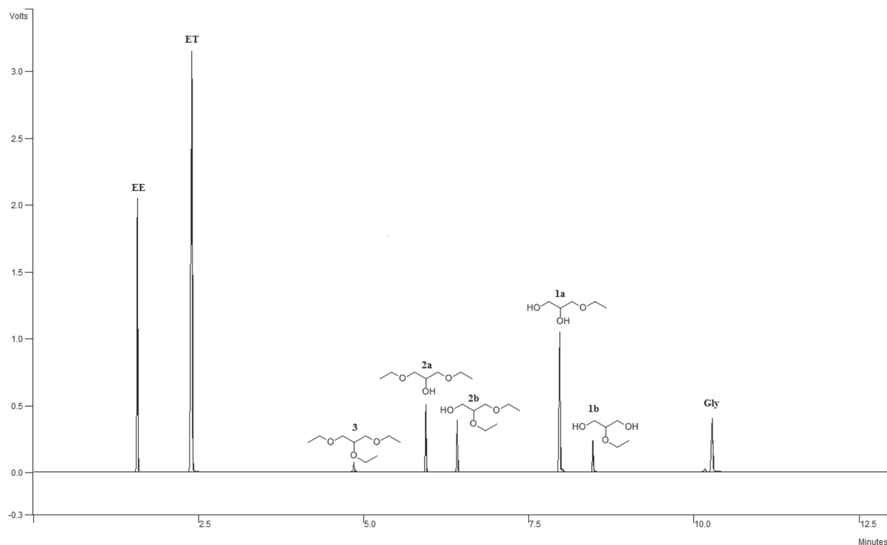
Figure 2. Chromatogram of the reaction medium of the etherification reaction of glycerol with ethanol. Peak identification: diethyl ether (EE); ethanol (ET); 1,2,3-triethoxy-propane ( 3 ); 1,3-diethoxy-propan-2-ol ( 2a ); 2,3-diethoxy-propan-1-ol ( 2b ); 3-ethoxy-propane-1,2-diol ( 1a ); 2-ethoxy-propane-1,3-diol ( 1b ); glycerol (Gly).
