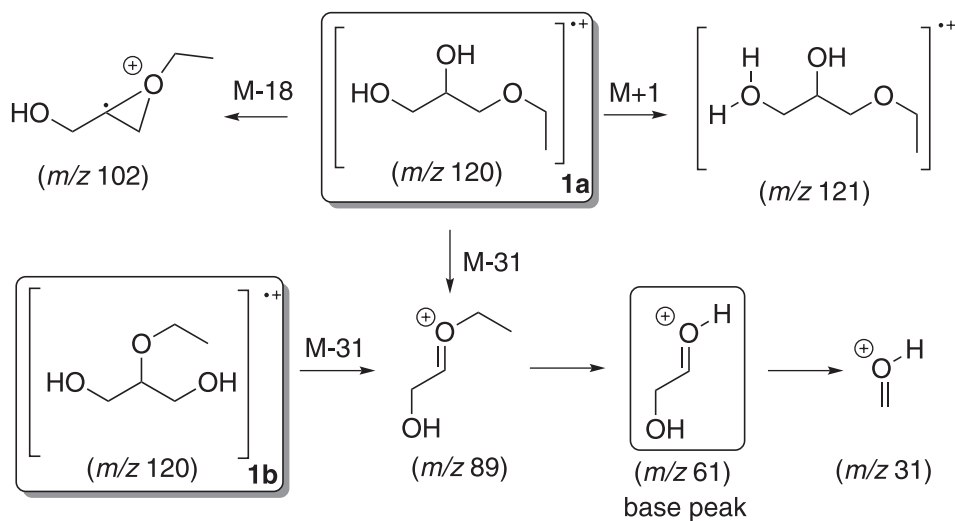
Figure 3. Proposed fragmentation pathway for 1a and 1b .
