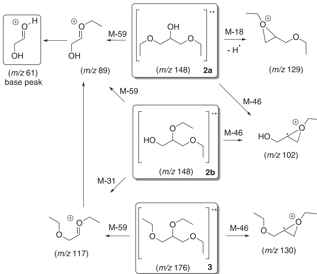
Figure 4. Proposed fragmentation pathway for diethers 2a and 2b and triether 3 .
