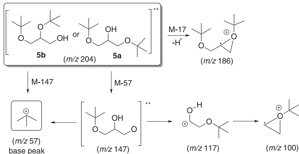
Figure 7. Proposed fragmentation pathway for disubstituted ethers 5a and 5b .
