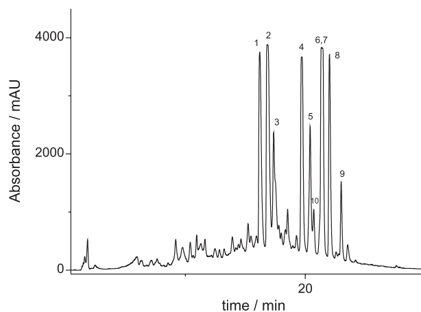
Figure 1. HPLC-UV chromatogram of ethanolic extract from citrus waste obtained after SPE clean-up. Peak numbers refer to compounds shown in Tables 1 and 2.
