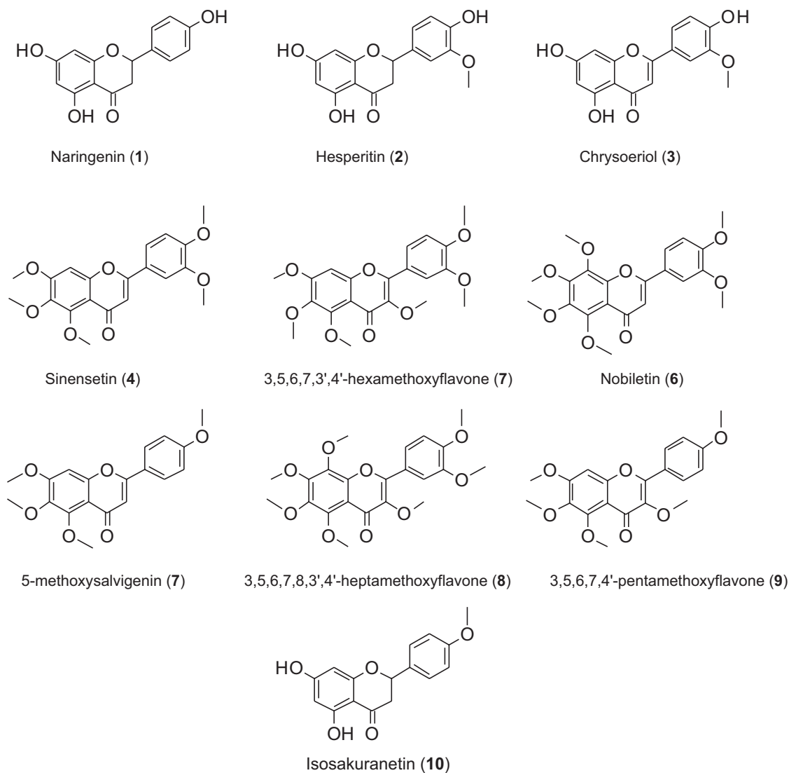
Figure 2. Flavonoid derivatives isolated from Brazilian citrus fruit processing wastes.
