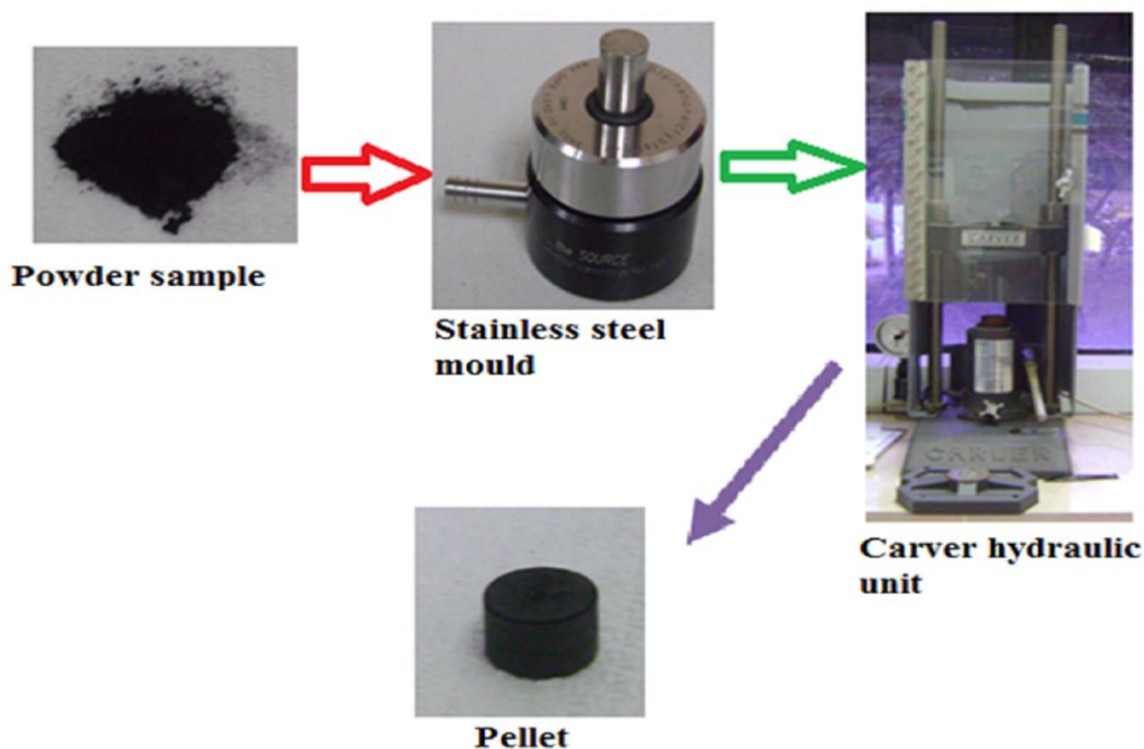
Figure S1. A full diagram for making a graphite-PVC composite pellet.
