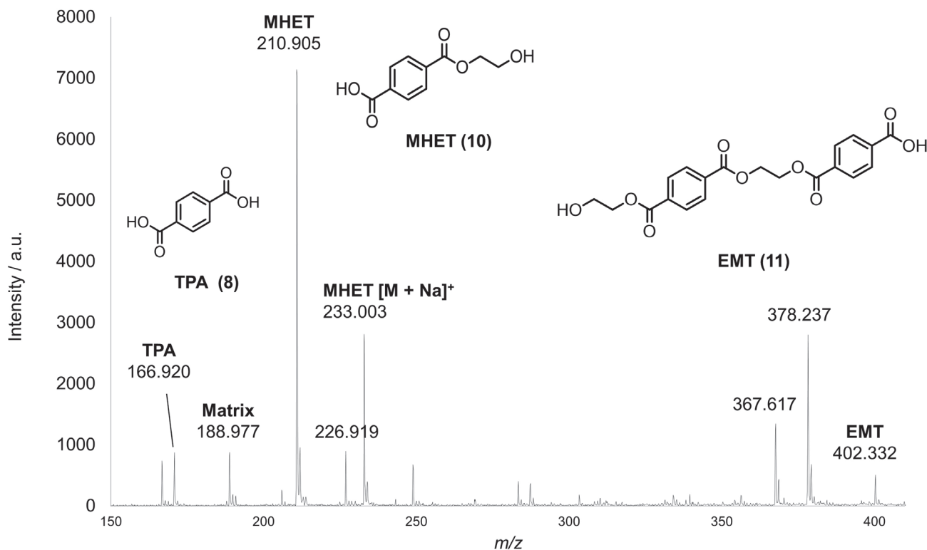
Figure 3. MALDI-TOF MS spectrum of the reaction medium for the second generation of the fungus Trichoderma sp. C70 after 15 days, detailing the peaks for hydrolysis products TPA, MHET and EMT.
