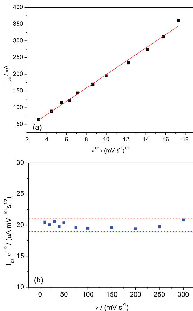
Figure 3. (a) Intensity of the anodic peak current ( I_{pa} ) as a function of the square root of the scan rate of the electrical potential ( v^{1/2} ); (b) plot of the current function ( I_{pa}/v^{1/2} ) versus the scan rate of the electrical potential in 1.00 mmol L -1 OXA solution, 0.100 mol L -1 KOH solution as supporting electrolyte and CPE. The dashed lines establish a maximal deviation of \pm 5.0\% from the mean value of the current function for all data.
