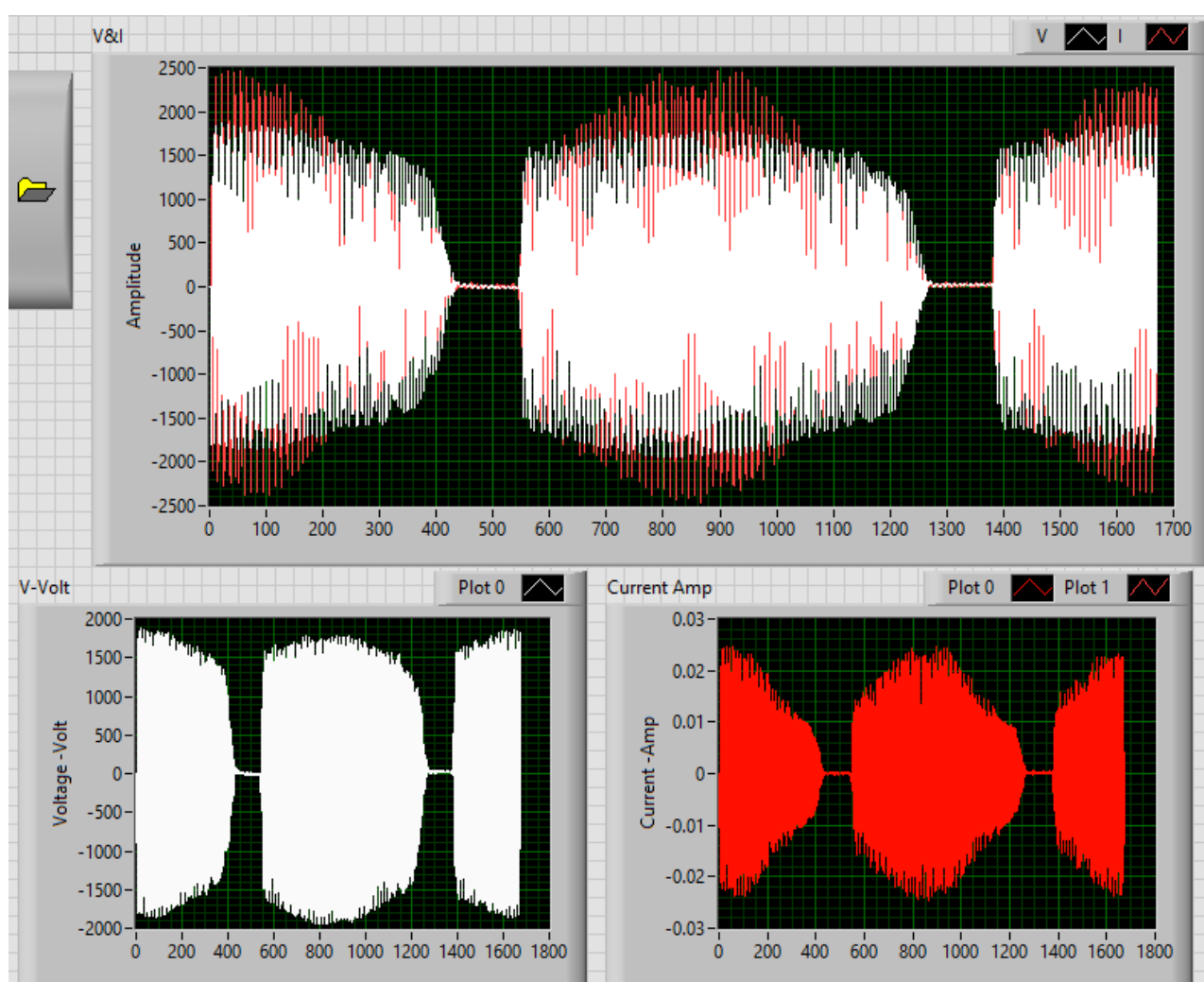
Figure S1. Waveform of current and voltage for the plasma system.
