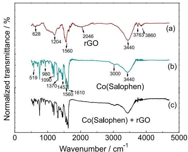
Figure 1. FTIR analyses of (a) graphene; (b) Co(Salophen); and (c) graphene/Co(Salophen).
