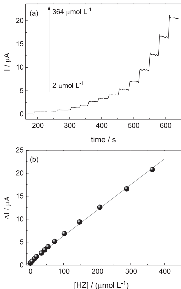
Figure 4. (a) Amperometric I-t curve for the determination of HZ at rGO/Co(Salophen)/DNA modified electrode; (b) analytical curve for the oxidation of HZ in 0.1 mol L -1 PBS at pH 7.0 for the concentrations: 2; 3; 7; 14; 20; 35; 45; 54; 74; 103; 148; 208; 288 and 364 μmol L -1 of HZ. E_{\text{appl.}} = 0.32 V.
