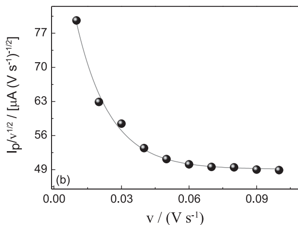
Figure 3. (a) Plot of peak current ( I_p ) versus the square root of scan rate for the rGO/Co(Salophen)/DNA modified electrode; (b) plot of ( I_p/v^{1/2} ) versus the scan rate. Date obtained from the Figure 3a: v = 0.01, 0.02, 0.03, 0.04, 0.05, 0.06, 0.07, 0.08, 0.09 and 0.1 V s -1 .
