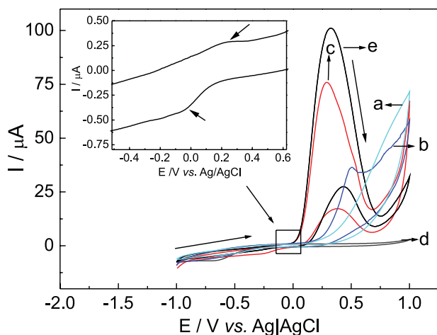
Figure 2. CVs of the bare (a) GCE; (b) rGO/DNA/GCE; and (c) Co(Salophen)/DNA/GCE in the presence of HZ. CVs of the rGO/Co(Salophen)/DNA/GCE: in (d) absence (voltammogram insert) and (e) presence of the HZ. Measurements were carried out in 0.1 mol L -1 PBS; pH 7; [HZ] = 0.3 mmol L -1 ; [Co(Salophen)] = 1 mmol L -1 ; [rGO] = 3 mg mL -1 ; [DNA] = 2 mg mL -1 ; v = 0.025 V s -1 .
