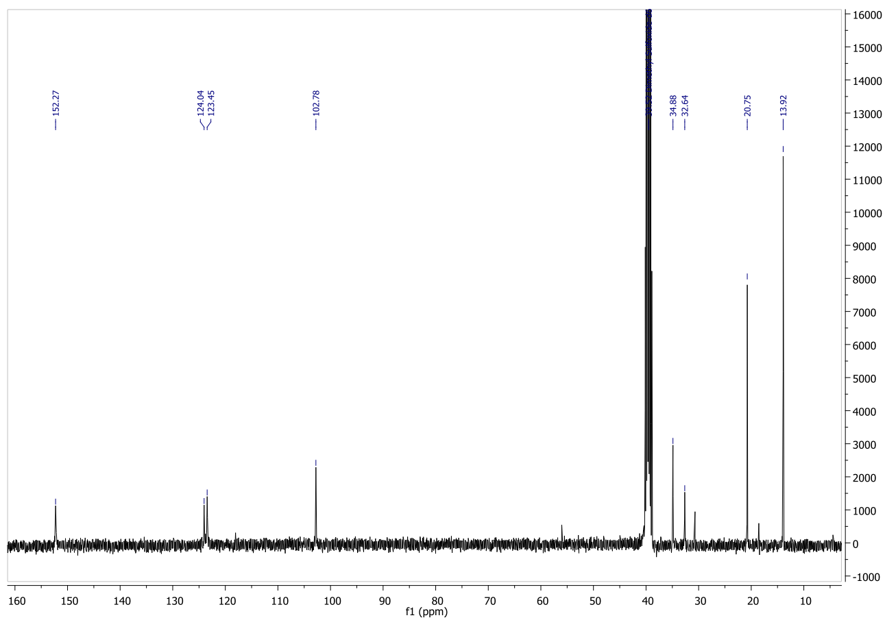
Figure S5. 13 C NMR spectrum (400 MHz, DMSO- d 6 , 303 K) of compound 5 .
