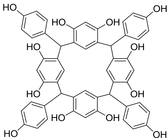
Figure S1. Structure of compound 4.
