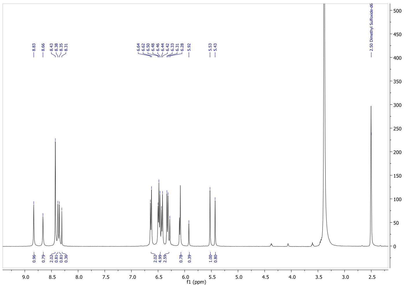
Figure S2. ^1\text{H} NMR spectrum (400 MHz, \text{DMSO-}d_6 , 303 K) of compound 4.
