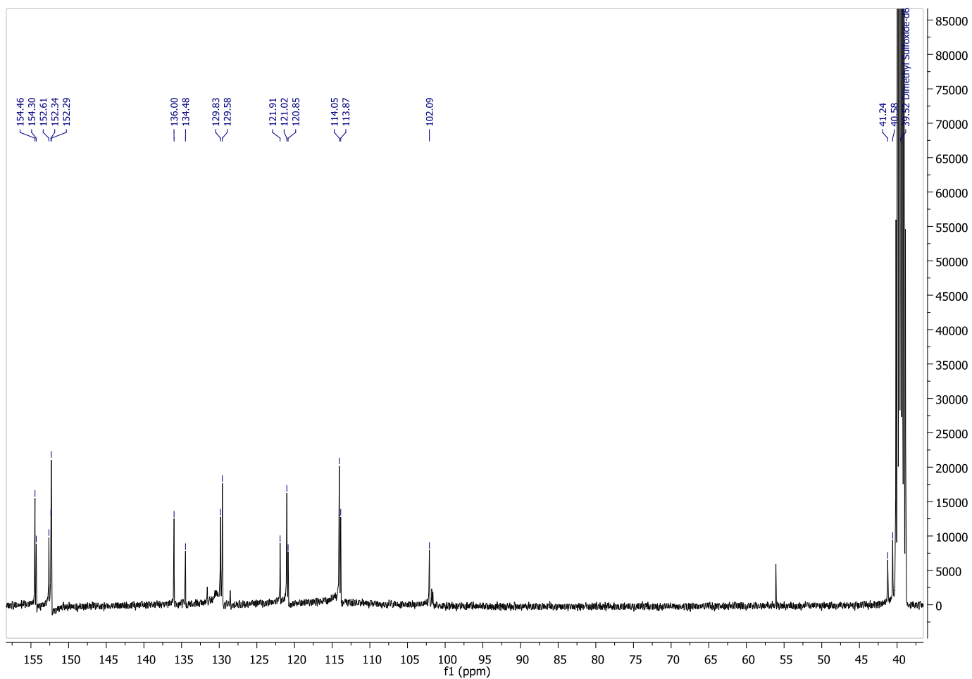
Figure S3. ^{13}\text{C} NMR spectrum (400 MHz, DMSO- d_6 , 303 K) of compound 4.
