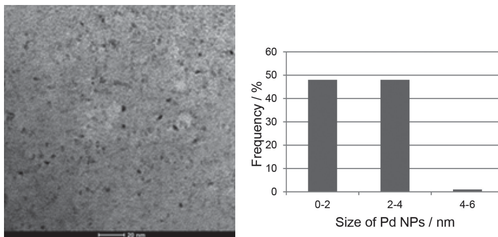
Figure 2. (Left) Image of 4.7% Pd on MgCO 3 and (right) its size distribution of nanoparticles (NPs) obtained by TEM analysis.
