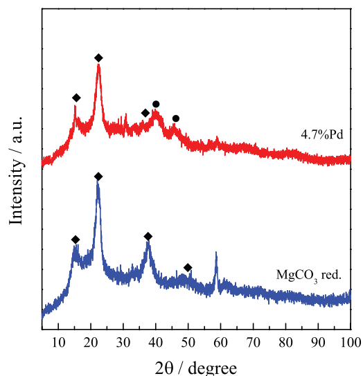
Figure 1. X-ray diffractogram of Pd/MgCO 3 catalyst.
