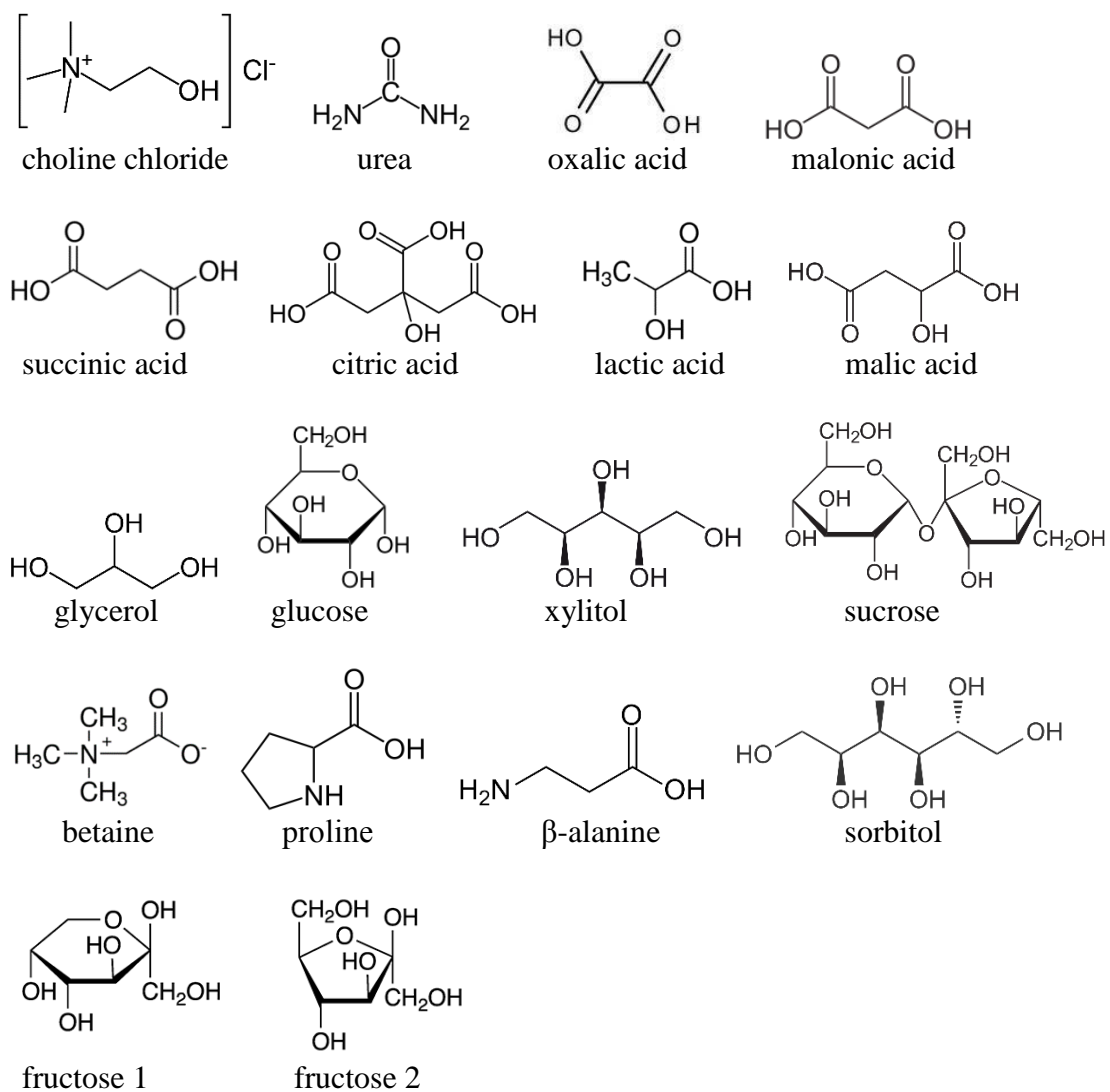
Figure S1. Chemical structures of components commonly used in natural deep eutectic solvents:
