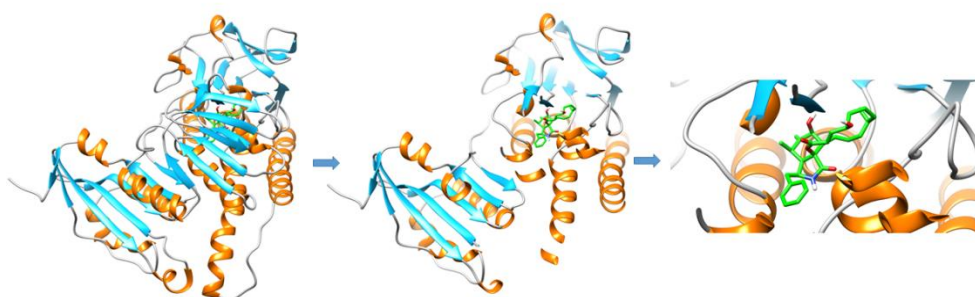
Figure S1. Conformation of the ligand (cytochalasin B) with better ELL and EI score.
