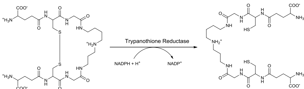
Figure S2. Representation of the participation of trypanothione reductase in the reduction of trypanothione disulfide in trypanothione dithiol.
