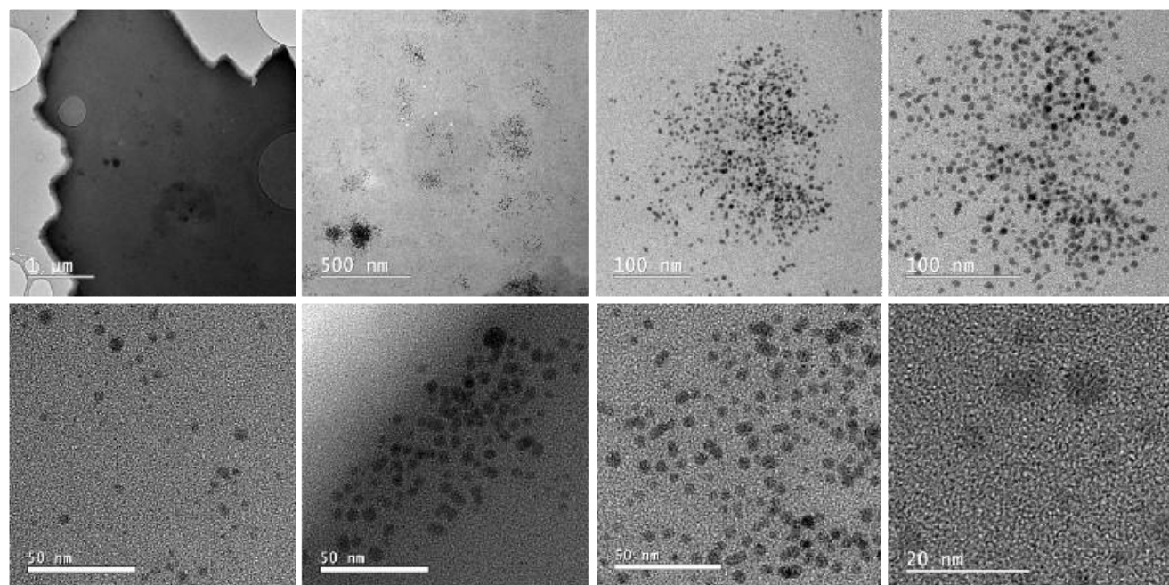
Figure S3. TEM images of Pd/TTH.
