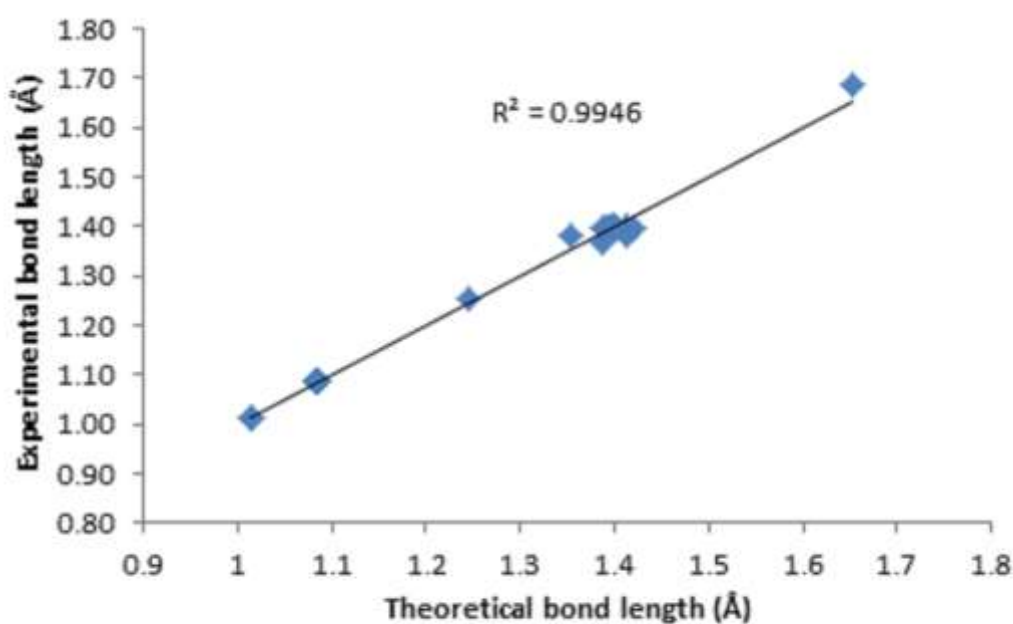
Figure S1. Calibration curve of experimental bond length against theoretical bond length.
