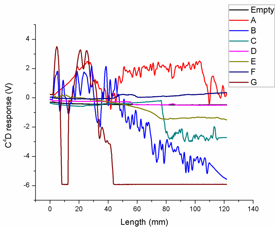
Figure S1. Scanning capacitively coupled contactless conductivity detection (SC 4 D) profiles for the synthesized columns.
