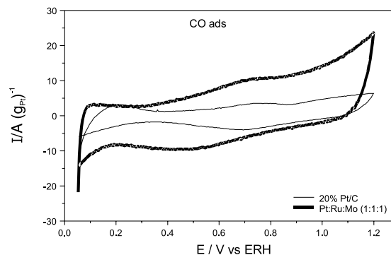
Figure 10. Cyclic voltammety of the catalyst systems in 0.5 \text{ mol L}^{-1} \text{ H}_2\text{SO}_4 and mixture \text{H}_2/\text{CO} 150 ppm with a sweep rate of 10 \text{ mVs}^{-1} .
