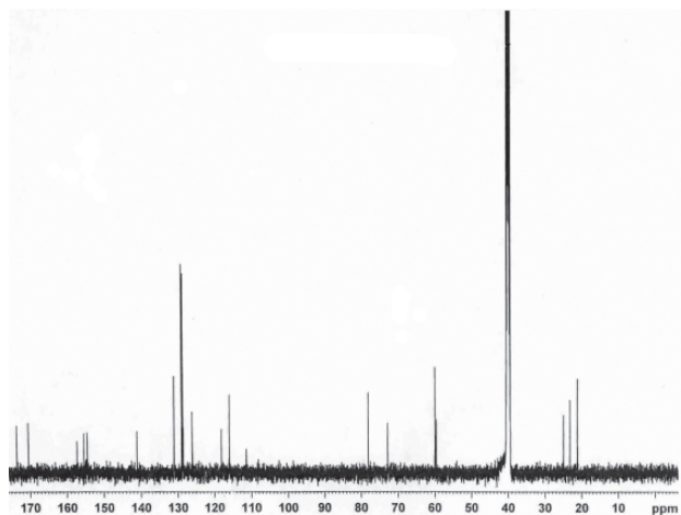
Figure S7. 13 C NMR spectra of 2.
