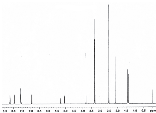
Figure S8. 1 H NMR spectra of 2.
