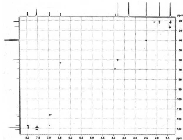
Figure S4. HSQC spectra of 1.
