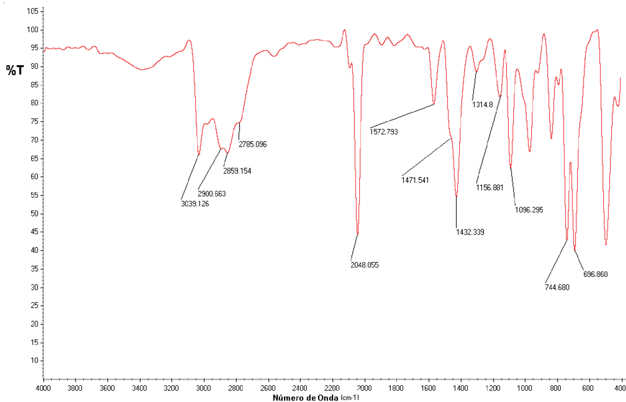
Figure S1. IR spectrum of the compound [Pd(C-dmba)(NCS)(dppp)] recorded as KBr pellets.
