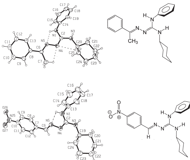
Figure 1. Crystal structures of 2a (top) and 2c (bottom). Displacement ellipsoids are drawn at the 30% probability level and H atoms are shown as spheres of arbitrary radii. The intramolecular H-bonds are shown with dashed lines.
