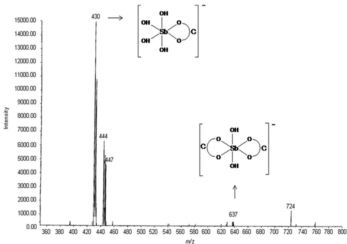
Figure S1. Negative ESI-MS spectrum of Sb V -C.
