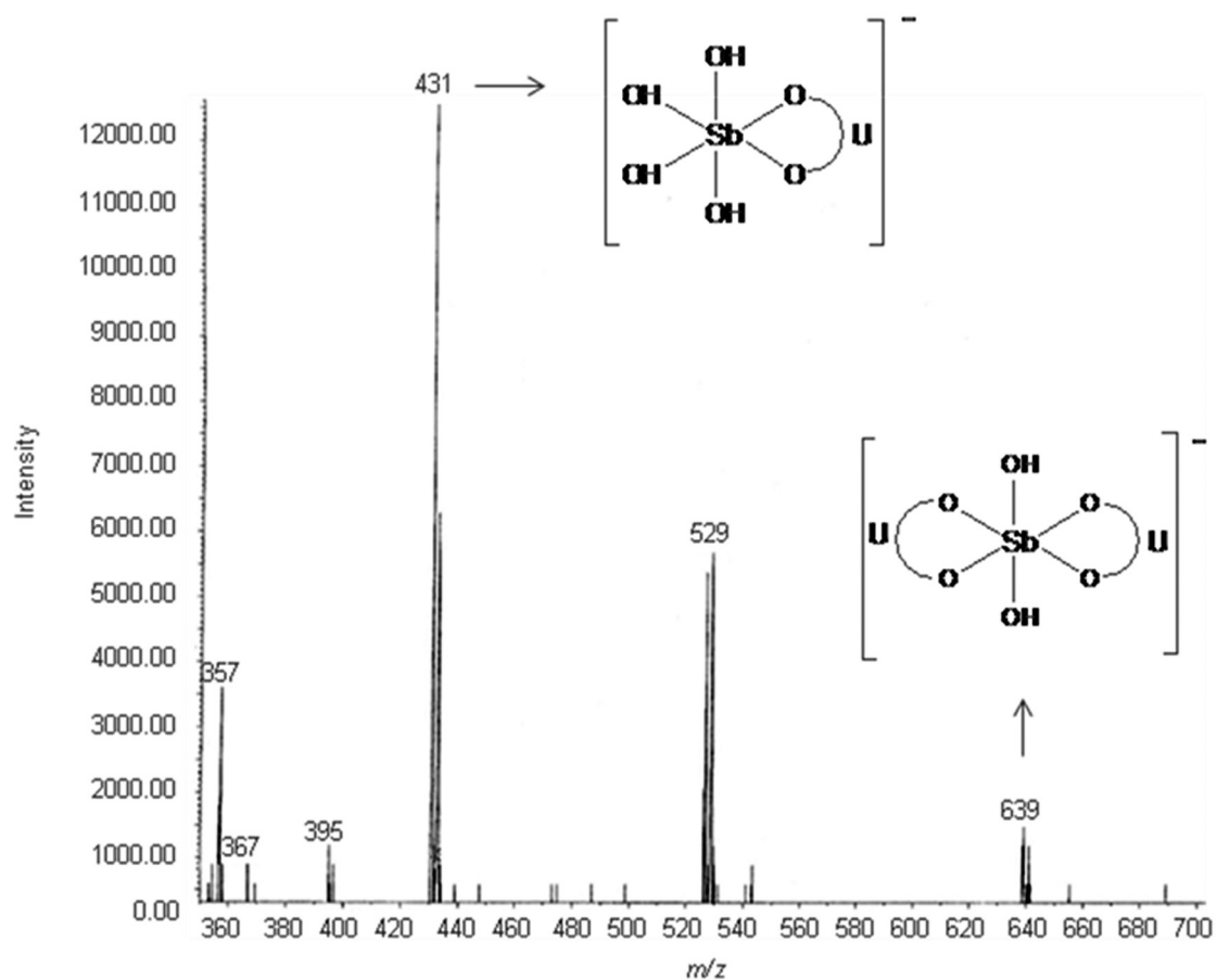
Figure S2. Negative ESI-MS spectrum of \text{Sb}^{\text{V}}\text{-U} .
