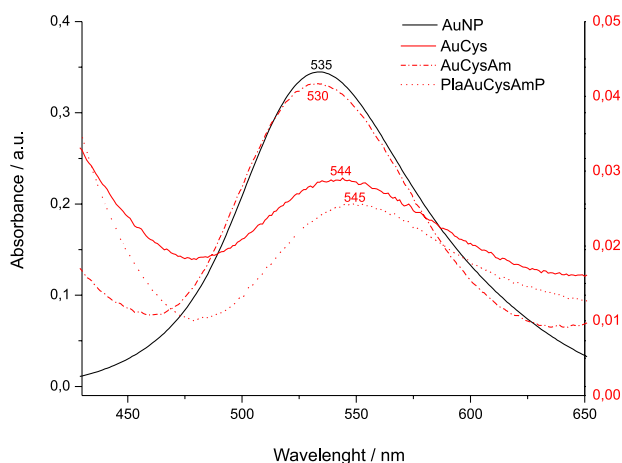
Figure S1. UV-Vis spectra of the nanoparticle suspensions: AuNP (reference, 535 nm), AuCys (Au with cysteine), AuCysAm (Au with cysteamine) and PLAAuCysAmPEG (Au with PLA, cysteamine and PEG-SH).
