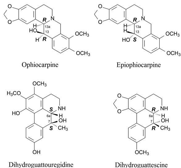
Figure 2. Structures of 13-hydroxytetrahydroprotoberberine alkaloids, (–)-ophiocarpine and (–)-epiophiocarpine, and 7-hydroxy-7-methylaporphine alkaloids, (–)-dihydroguattouregidine and (+)-dihydroguattescine, showing their absolute configurations.
