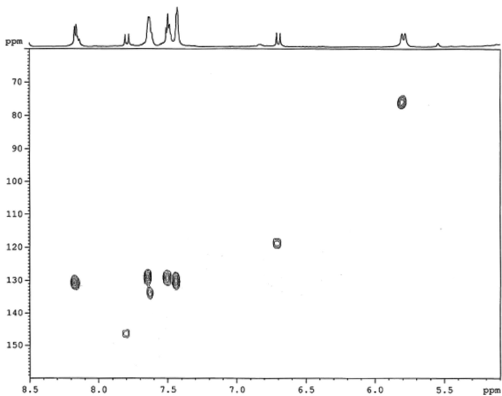
Figure S2. HSQC spectrum of compound 1 (600 MHz, CD 3 OD).
