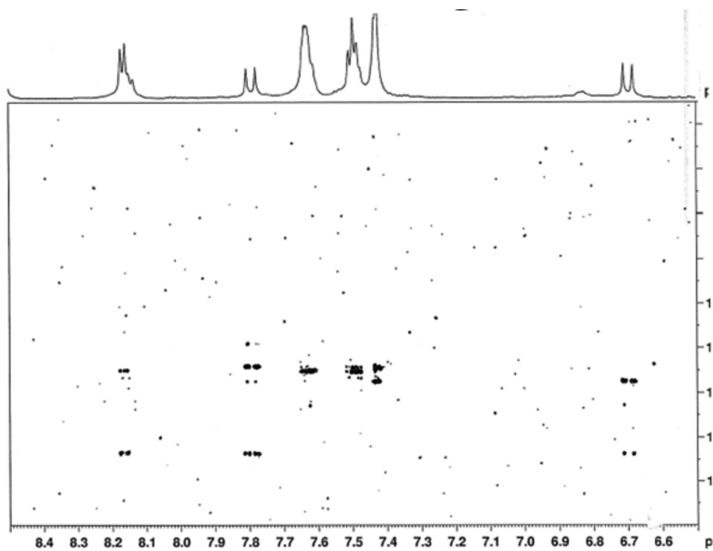
Figure S3. HMBC spectrum of compound 1 (600 MHz, CD 3 OD).
