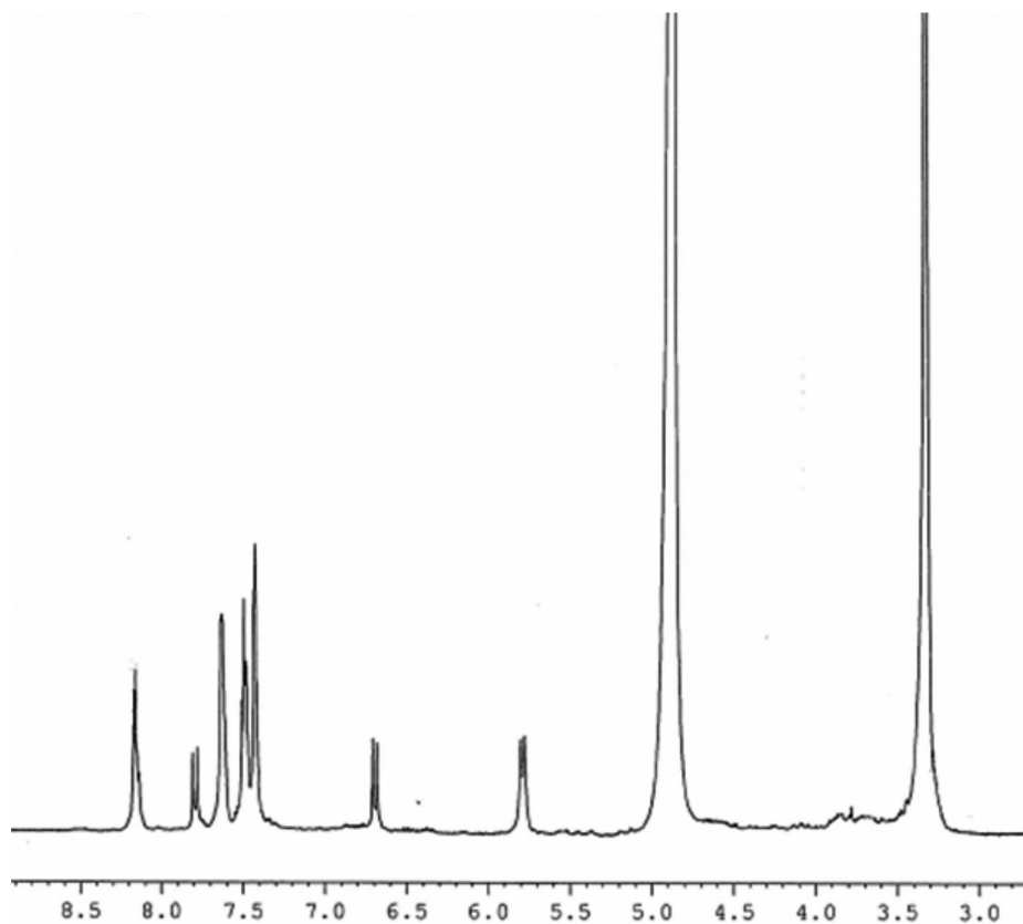
Figure S1. 1 H NMR spectrum of compound 1 (600 MHz, CD 3 OD).
