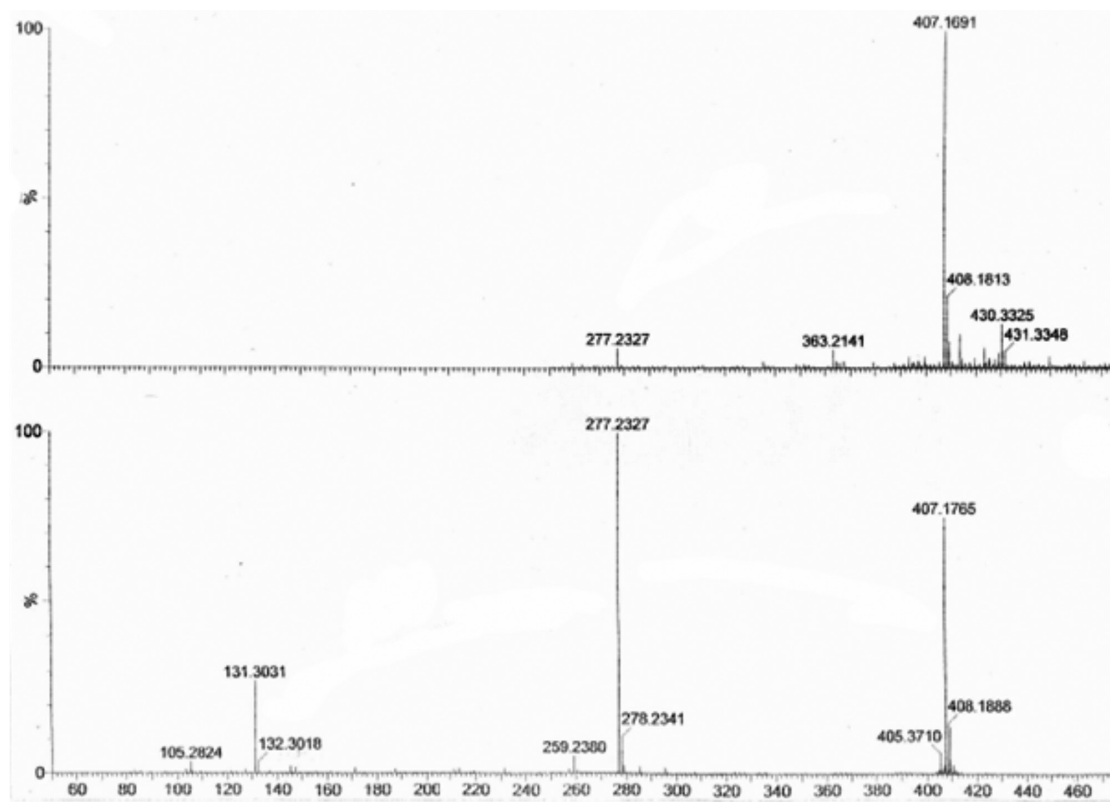
Figure S4. HR-ESI-MS spectrum of compound 1.
