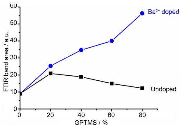
Figure S1. Area of the most intense phosphotungstate IR absorption band (ca. 821 cm -1 ) as function of % GPTMS for the Ba 2+ doped and undoped hybrid films.
