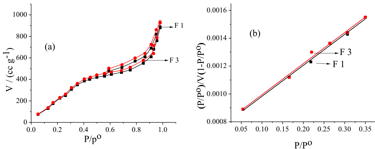
Figure S4. Nitrogen adsorption/desorption isotherms (a) and linear BET plot (b) at -196\text{ }^{\circ}\text{C} onto F1 and F3.
