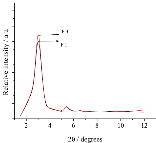
Figure S3. XRD patterns for F1 and F3.
