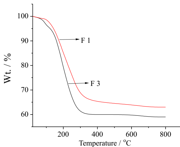
Figure S2. TGA for F1 and F3.
