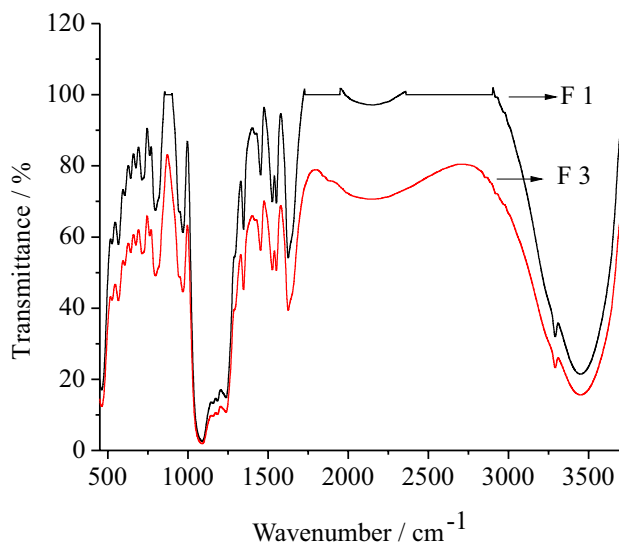
Figure S1. FTIR (KBr) spectra for F1 and F3.
