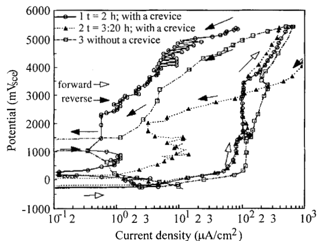
Figure 5. Discontinuous (for creviced sample) and continuous (for uncreviced sample) cyclic voltammetric curves at 90 °C in neutral and aerated 1 M NaCl. The forward scan was at v = 1200 mV/min, and the reverse at 120 mV/min for the discontinuous curves; the forward and reverse scans were at v = 1200 mV/min for the continuous curve. Hold at +5300 mV for 120 min (curve 1) and 200 min (curve 2), and no hold (curve 3).
