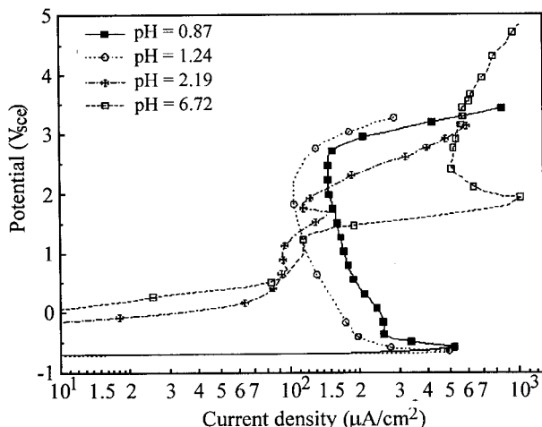
Figure 2. Potentiodynamic curves for different pHs after spontaneous activation in deaerated 1 M NaCl, scan rate v = 1200 mV/min; T = 90 °C.
