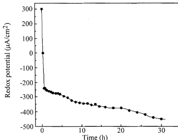
Figure 4. Variation of the redox potential of a deaerated 1 M NaCl solution, pH = 1, in the presence of Ti filings ( T = 90 °C).
