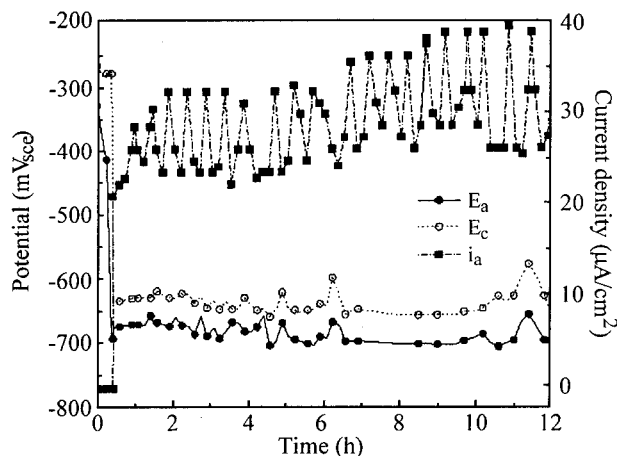
Figure 3. Variation of the anodic and cathodic potential and the anodic current density in electrochemical simulation tests of crevice corrosion in a two-compartment cell ( T = 90 °C, 1 M NaCl, and A_c/A_a = 0.6 ).
