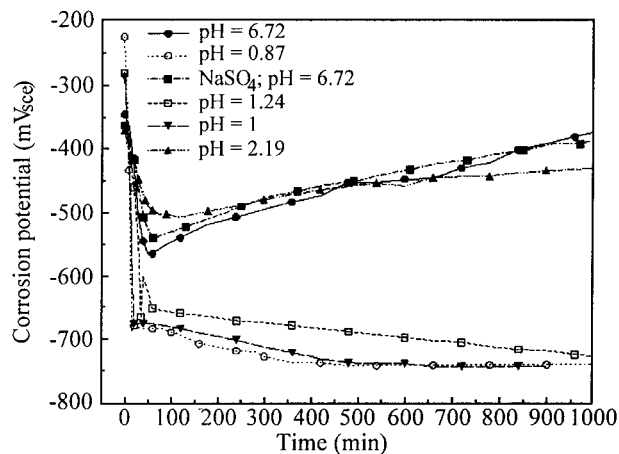
Figure 1. Spontaneous activation curves for uncreviced Ti samples in a deaerated medium for several pHs; T = 90 °C, 1 M NaCl.
