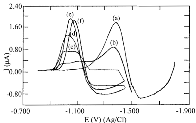
Figure 2. Differential pulse polarograms for 1 \times 10^{-3} mol/L cobalt(II) solution at ionic strength 2.0 mol/L with azide concentrations: (a) 0, (b) 0.05, (c) 0.10, (d) 0.20, (e) 1.0, and (f) 2.0. Scan rate: 10 \text{ mV s}^{-1} ; scan increment: 2 mV; pulse width: 50 ms; pulse height: 25 mV.
