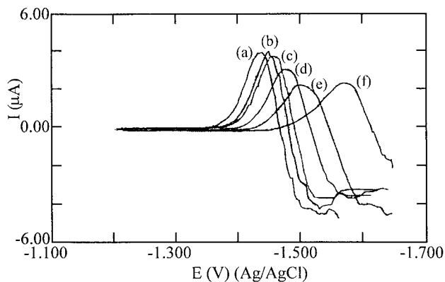
Figure 6. Differential pulse polarograms for 1 \times 10^{-3} mol/L manganese(II) solution at ionic strength 2.0 mol/L with azide concentrations: (a) 0, (b) 0.10, (c) 0.20, (d) 0.50, (e) 1.0, and (f) 2.0. Scan rate: 10 \text{ mV s}^{-1} ; scan increment: 2 mV; pulse width: 50 ms; pulse height: 25 mV.
