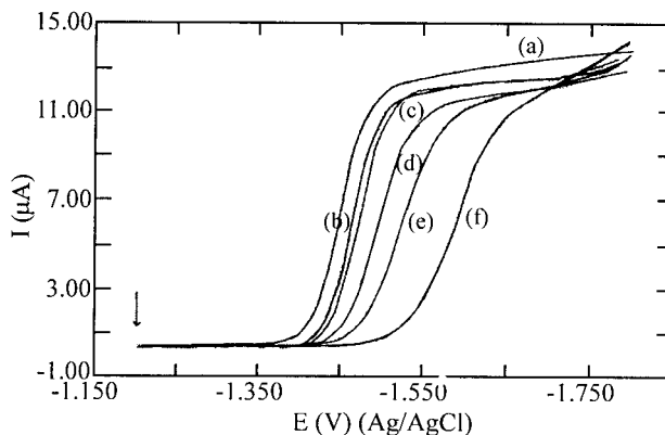
Figure 5. Normal pulse polarograms for 1 \times 10^{-3} mol/L manganese(II) solution at ionic strength 2.0 mol/L with azide concentrations: (a) 0, (b) 0.10, (c) 0.20, (d) 0.50, (e) 1.0, and (f) 2.0. Initial potential: -1.2 V; scan rate: 10 \text{ mVs}^{-1} ; scan increment: 2 mV; pulse width: 50 ms.
