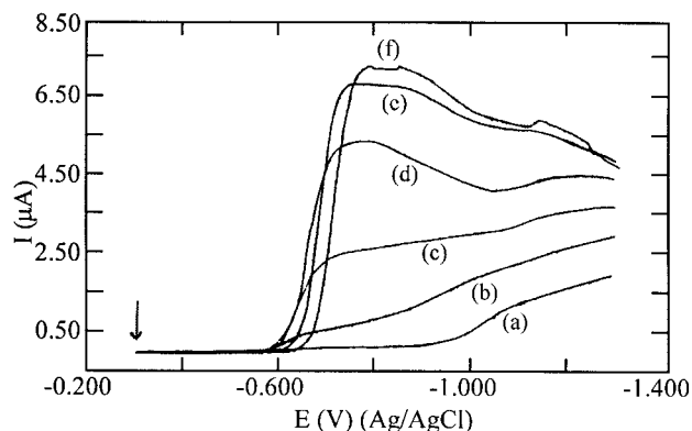
Figure 3. Normal pulse polarograms for 0.5 \times 10^{-3} mol/L nickel(II) solution at ionic strength 2.0 mol/L with azide concentrations: (a) 0, (b) 0.05, (c) 0.10, (d) 0.20, (e) 1.0, and (f) 2.0. Initial potential: -0.3 V, scan rate: 10 \text{ mVs}^{-1} ; scan increment: 2 mV; pulse width: 20 ms.
