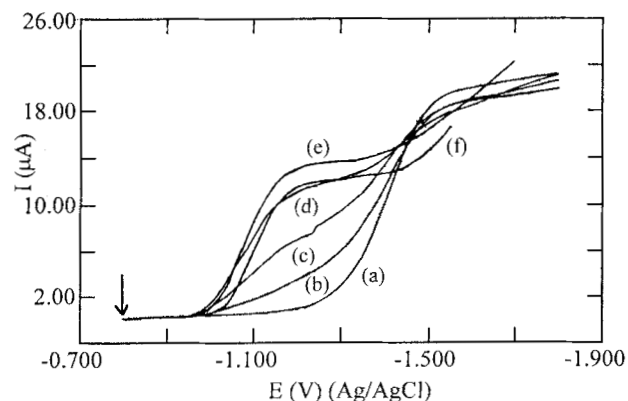
Figure 1. Normal pulse polarograms for 1 \times 10^{-3} mol/L cobalt(II) solution at ionic strength 2.0 mol/L with azide concentrations: (a) 0, (b) 0.05, (c) 0.10, (d) 0.20, (e) 1.0, and (f) 2.0. Initial potential: -0.8 V; scan rate: 10 \text{ mV s}^{-1} ; scan increment: 2 mV; pulse width: 50 ms.
