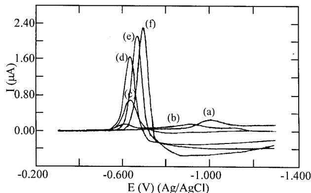
Figure 4. Differential pulse polarograms for 0.5 \times 10^{-3} mol/L nickel(II) solution at ionic strength 2.0 mol/L with azide concentrations: (a) 0, (b) 0.05, (c) 0.10, (d) 0.20, (e) 1.0, and (f) 2.0. Scan rate: 10 \text{ mVs}^{-1} ; scan increment: 2 mV; pulse width: 20 ms; pulse height: 25 mV.
