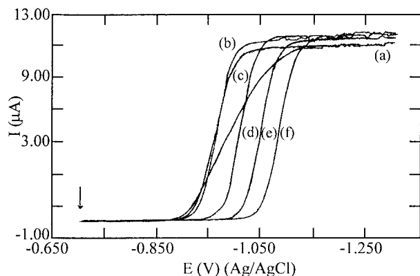
Figure 7. Normal pulse polarograms for 1 \times 10^{-3} mol/L zinc(II) solution at ionic strength 2.0 mol/L with azide concentrations: (a) 0, (b) 0.03, (c) 0.10, (d) 0.50, (e) 1.0, and (f) 2.0. Initial potential: -0.7 \text{ V} ; scan rate: 10 \text{ mV s}^{-1} ; scan increment: 2 mV; pulse width: 50 ms.
