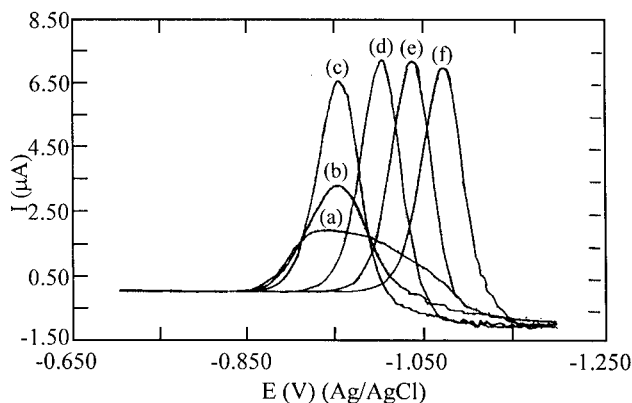
Figure 8. Differential pulse polarograms for 1 \times 10^{-3} mol/L zinc(II) solution at ionic strength 2.0 mol/L with azide concentrations: (a) 0, (b) 0.03, (c) 0.10, (d) 0.50, (e) 1.0, and (f) 2.0. Scan rate: 10 \text{ mV s}^{-1} ; scan increment: 2 mV; pulse width: 50 ms; pulse height: 25 mV.
