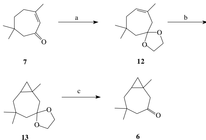
Scheme 3. Reaction conditions: (a) \text{HOCH}_2\text{CH}_2\text{OH} , Benzene, \text{PTSA} , reflux, 15h (85%); (b) Benzene, \text{Et}_2\text{Zn} , \text{CH}_2\text{I}_2 , 40^{\circ}\text{C} ; \text{O}_2 , 1h (89%); (c) Acetone, \text{PTSA} , 20^{\circ}\text{C} , 2h (97%).
