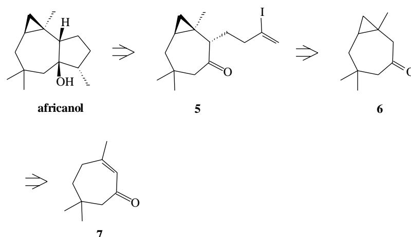
Scheme 1. Retrosynthetic analysis of africanol.
