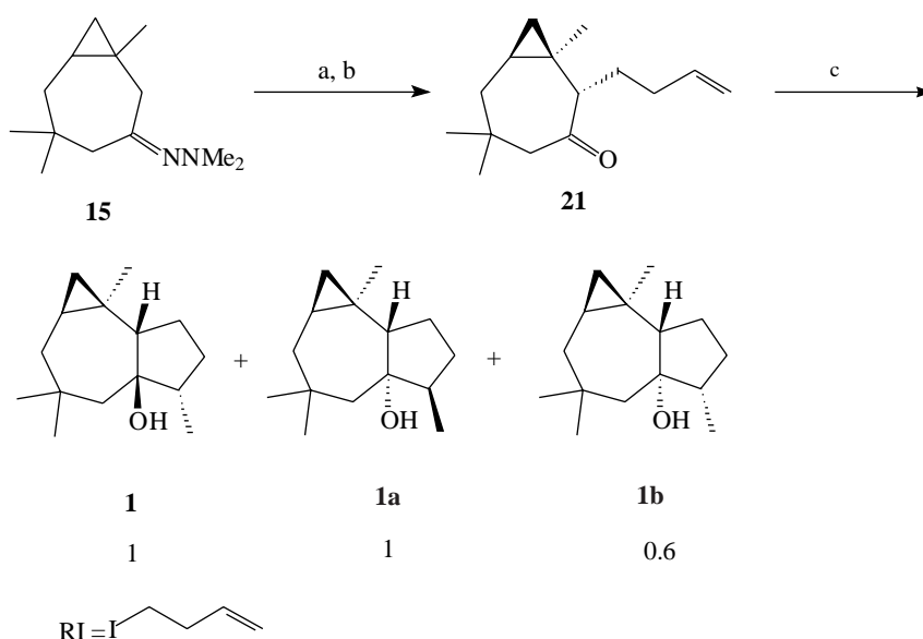
Scheme 6. Reaction conditions: (a) THF, LDA, 0°C, 2h; RI, 0°C→20°C, 17 h; (b) HOAc, THF, H 2 O, NaOAc (15:2:2:1 w/w) (50% from 15); (c) THF, HMPA, SmI 2 , t-BuOH, 20°C, 28 h (60%).
